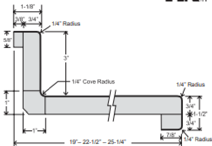
KITCHEN & VANITY TOP CNV 19 CNV 22-1/2 CNK 25-1/4
