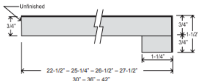
FLAT DECK TOP DFF 22-1/2 DFF 25-1/4 DFF 26-1/2 DFF 27-1/2 DFF 30 DFF 36 DFF 42
