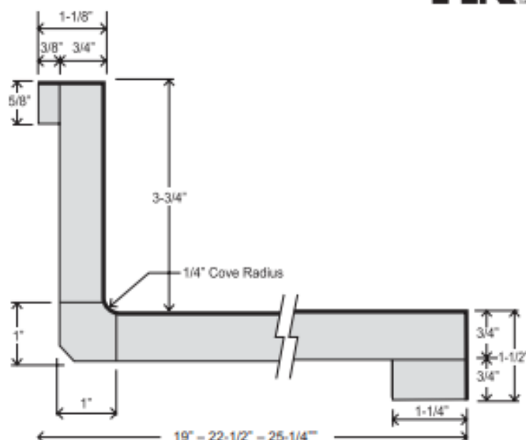
KITCHEN & VANITY TOP DFV 19 DFV 22-1/2 DFK 25-1/4
